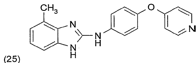
(4-Methyl-1H-benzimidazol-2-yl)-[4-(pyridin-4-yloxy)-phenyl]-amin
